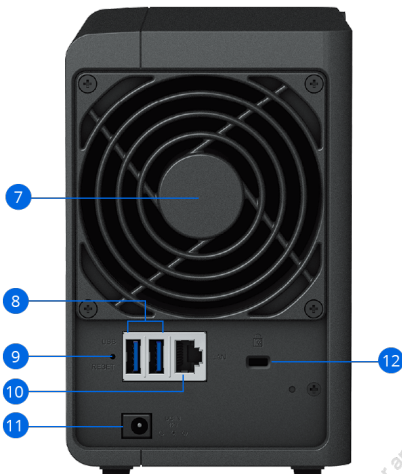
DS223 (Rear)
